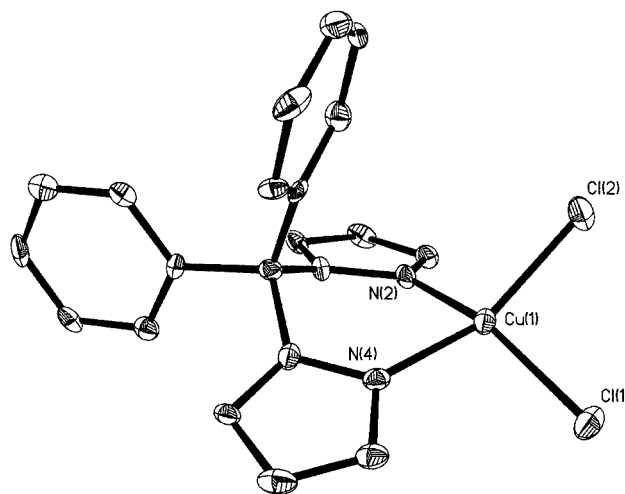
Figure 6. Structure of compound 8 with hydrogens omitted for clarity and thermal ellipsoids drawn at 50 % probability
