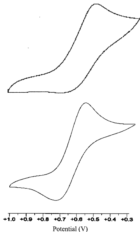
Figure 9. Cyclic voltammograms of compounds 4 (top) and 5 (bottom) at a scan rate of 50 mV/s in \text{CH}_3\text{CN} with 0.1 M [\text{Bu}_4\text{N}]\text{BF}_4 vs. SCE; y-axis is current measured in \mu\text{A}
