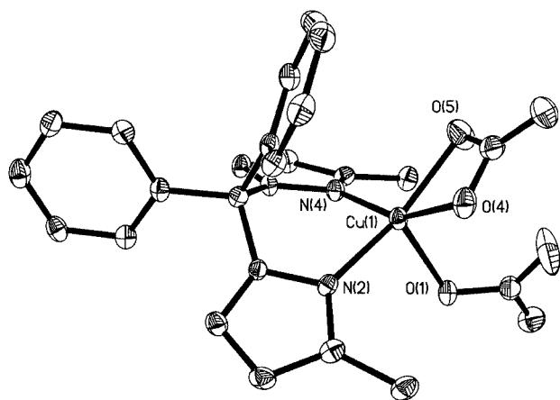
Figure 4. Structure of compound 5 with hydrogens omitted for clarity and thermal ellipsoids drawn at 50 % probability
