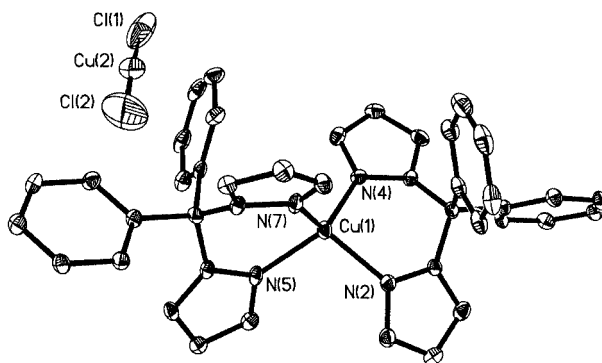
Figure 5. Structure of compound 7 with hydrogens omitted for clarity and thermal ellipsoids drawn at 50 % probability
