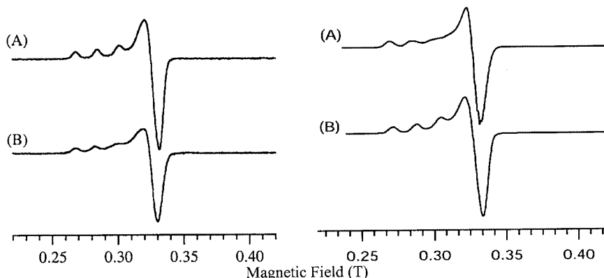
Figure 8. EPR spectra of compounds 4 (top, left), 5 (bottom, left), 6 (top, right) and 8 (bottom, right) (9.42 GHz) in MeOH at 120 K
