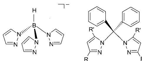
Figure 1. Schematic drawings of the ligands tris(pyrazolyl)borate (left) and diphenyldipyrzolylmethane (right) where R = R' = H ( 1 ), R = R' = CH_3 ( 2 ) and R = CH_3 , R' = H ( 3 )
