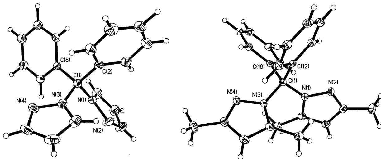
Figure 2. Structures of compounds 1 and 2 with thermal ellipsoids drawn at 50 % probability
