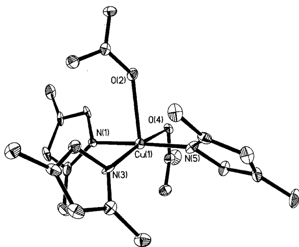
Figure 7. Structure of compound 6 with hydrogens omitted for clarity and thermal ellipsoids drawn at 50 % probability
