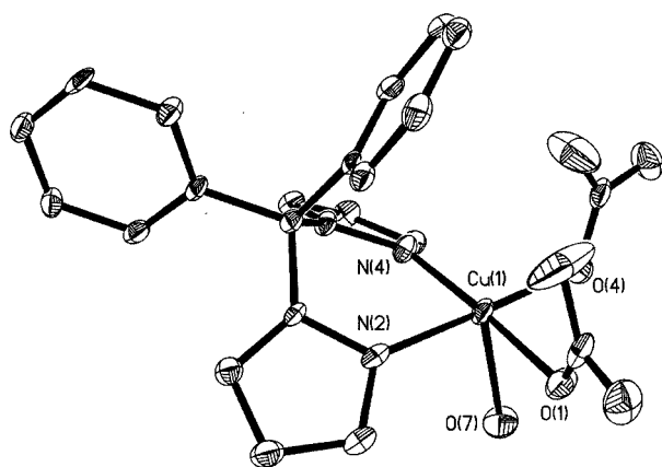
Figure 3. Structure of compound 4 with hydrogens omitted for clarity and thermal ellipsoids drawn at 50 % probability
